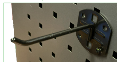
428.8552.01 lateral hooks
